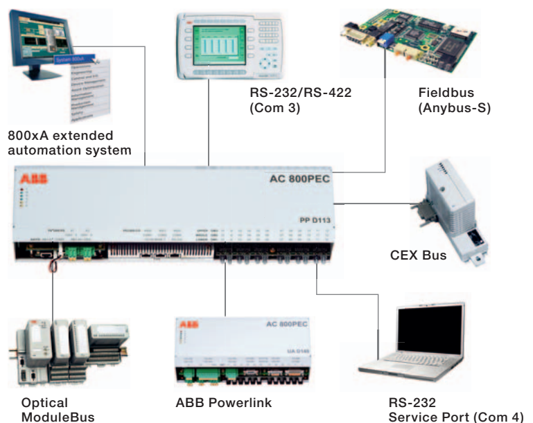
AC 800PEC connectivity: from overall plant control down to the process
