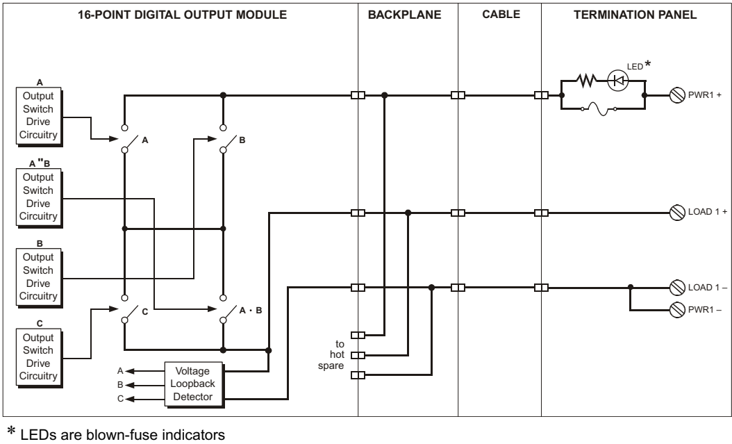
Figure 97 Simplified Schematic of a 3604E DO Module with a Non-Commoned DO Panel
