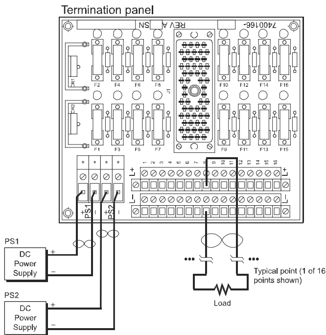
Figure 82 Field Wiring for 9664-810 with a 3603E or 3603T Module
