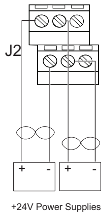
Figure 181 Power Wiring for 9764-310
