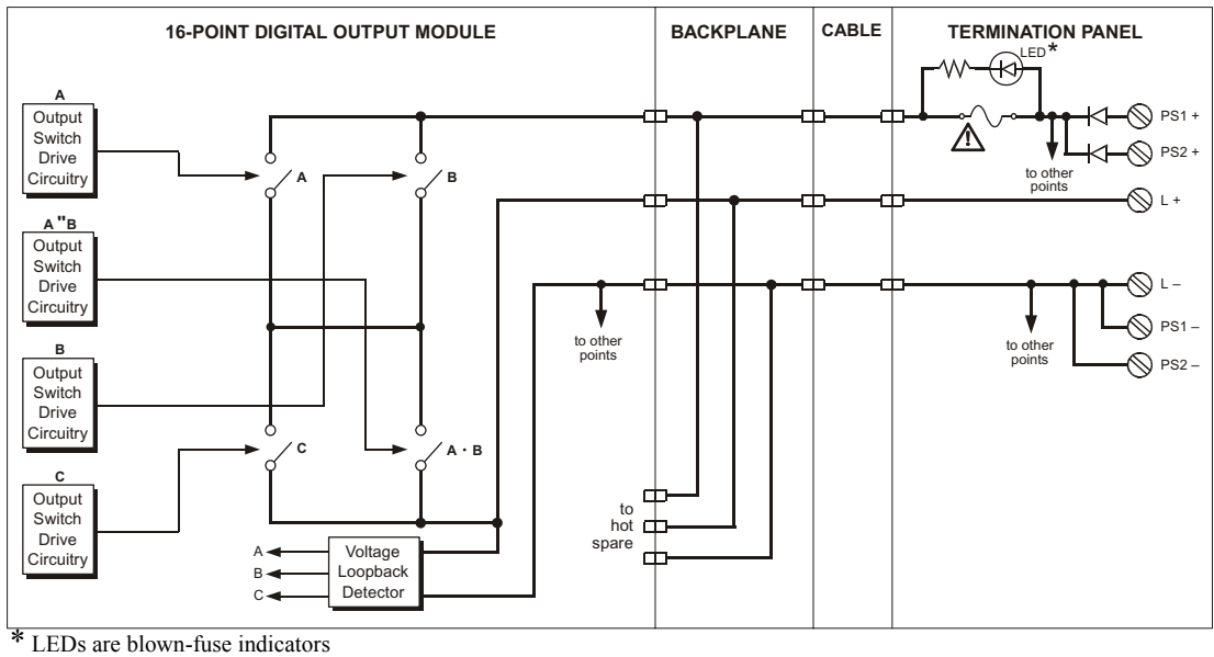
Figure 81 Simplified Schematic of a 3601E or 3601T DO Module with a Commoned DO Panel
