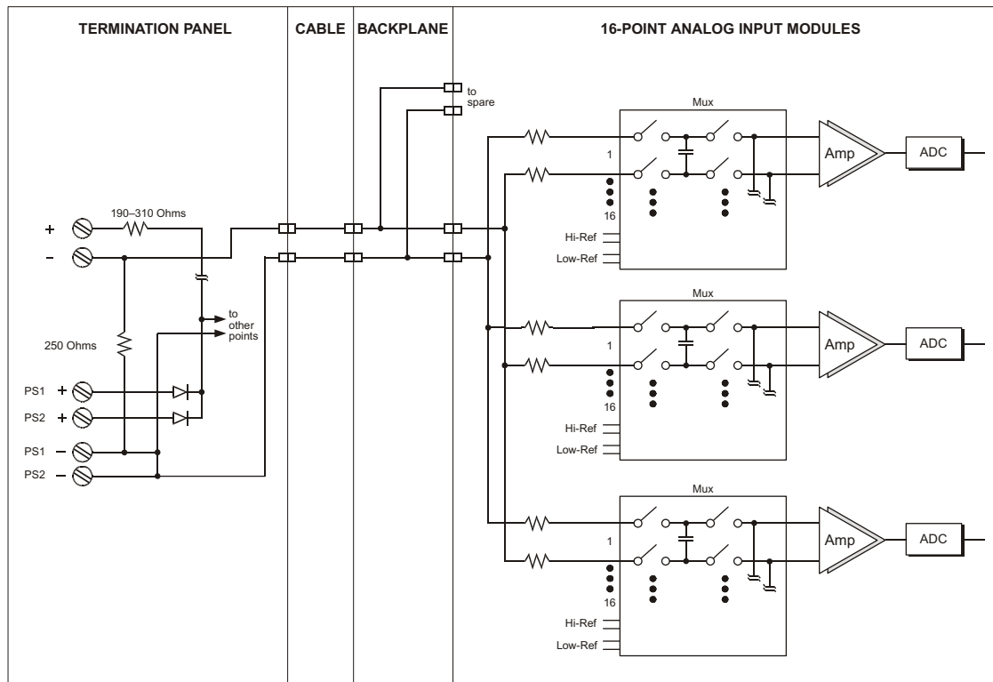
Figure 238 Simplified Schematic of a 3703E Analog Input Module with a 9795-610 Panel
