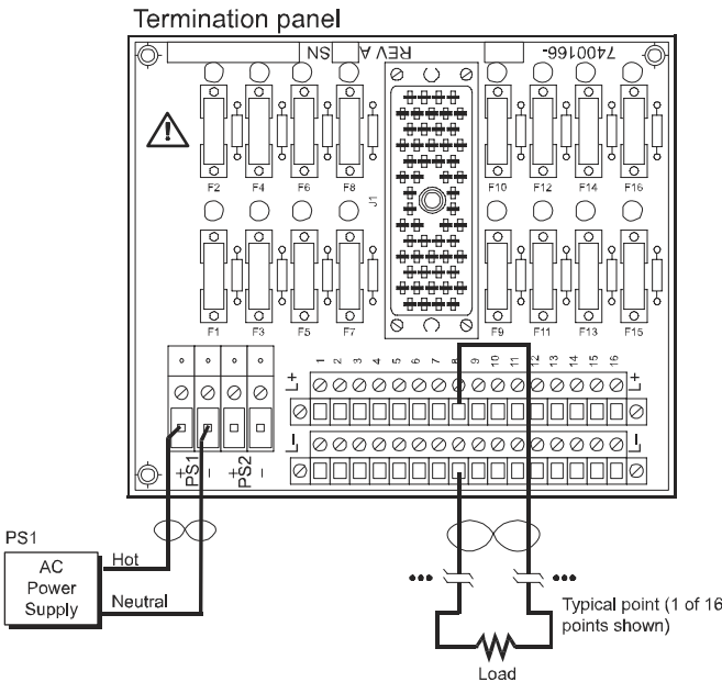
Figure 67 Field Wiring for 9661-610 with a 3601E Module
