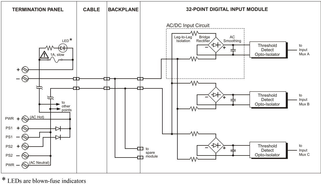
Figure 5 Simplified Schematic of a 3501E or 3501T DI Module with a 9561-810 Panel
