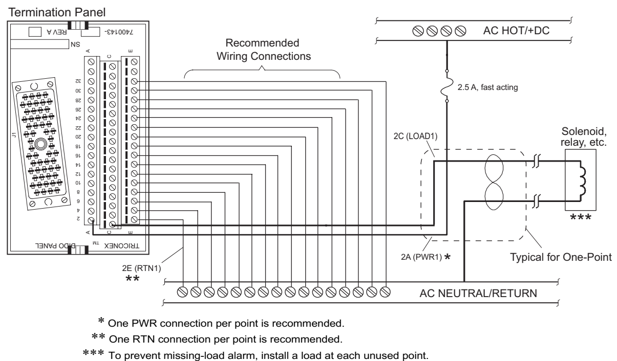
Figure 113 Field Wiring for 9653-610 with a 3604E DO Module
