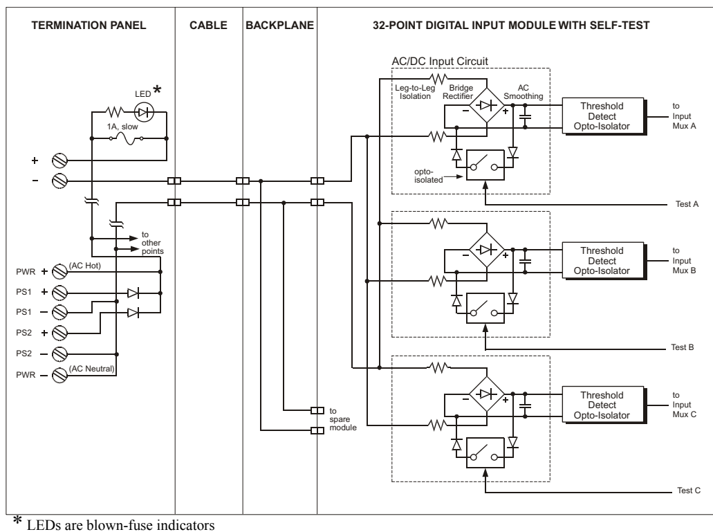
Figure 7 Simplified Schematic of a 3502E DI Module with a 9562-810 Panel
