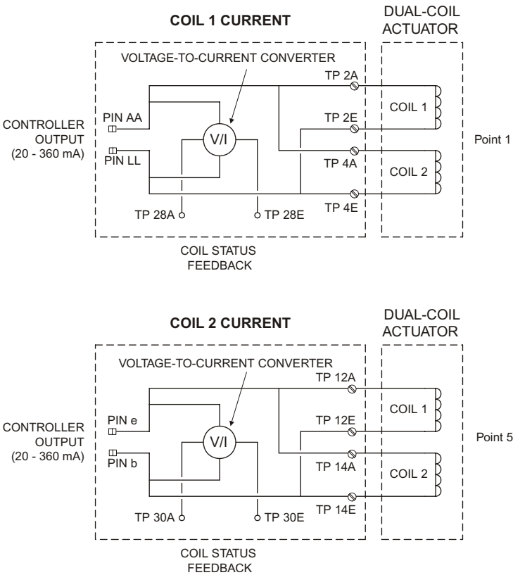
Figure 189 High-Current Circuits
