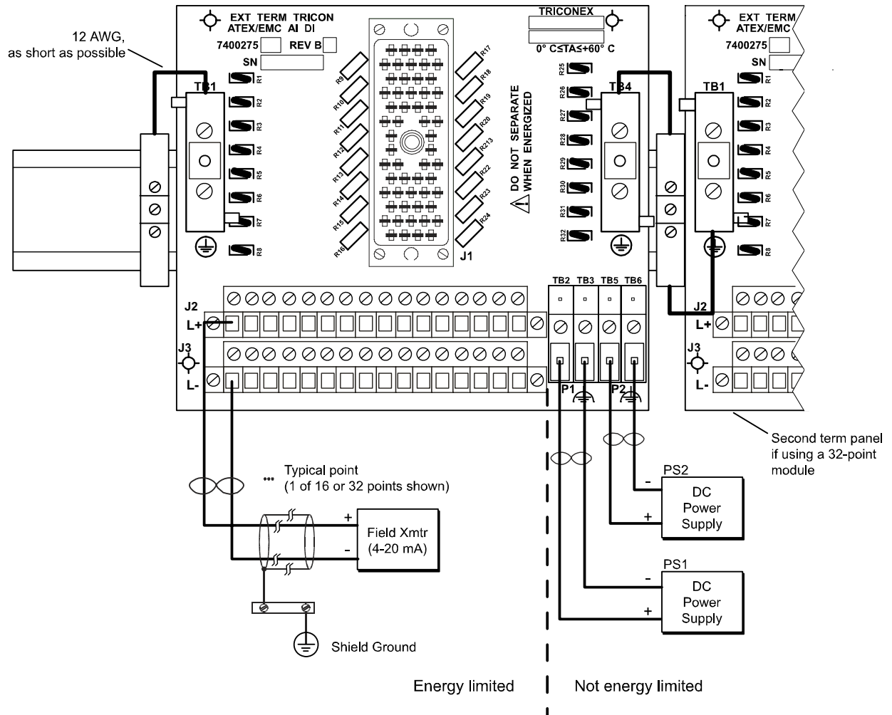
Figure 232 Field Wiring for 9790-610 with a 3700A, 3703E, or 3721 AI Module or 2770H HART AI Interface Module
