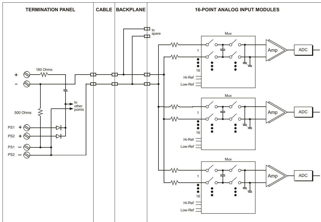
Figure 143 Simplified Schematic of a 3703E AI Module with a 9762-410 Panel
