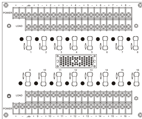
Figure 88 Typical 16-Point Non-Commoned DO Term Panel for Module 3603B
