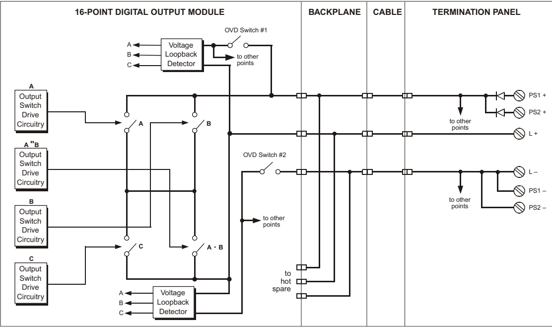
Figure 75 Simplified Schematic of a 3624 DO Module with a Commoned DO Panel
