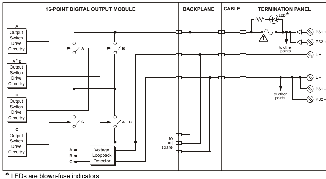
Figure 87 Simplified Schematic of a 3607E DO Module with a Commoned DO Panel
