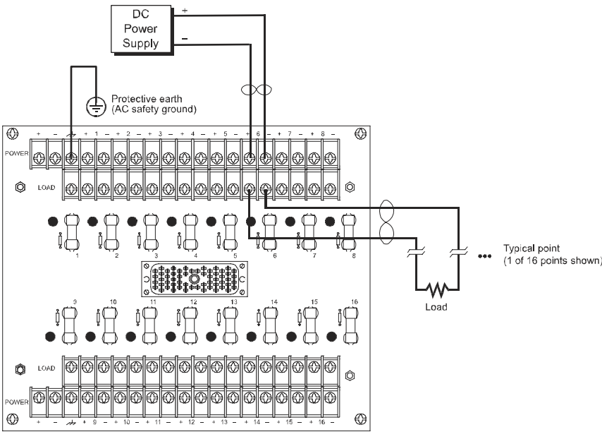
Figure 92 Field Wiring for 9251-210 with a 3603B Module
