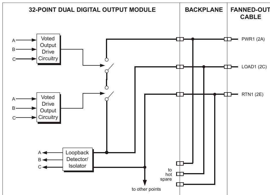
Figure 266 Simplified Schematic of a 3664 or 3674 DO Module with a Fanned-Out Cable
