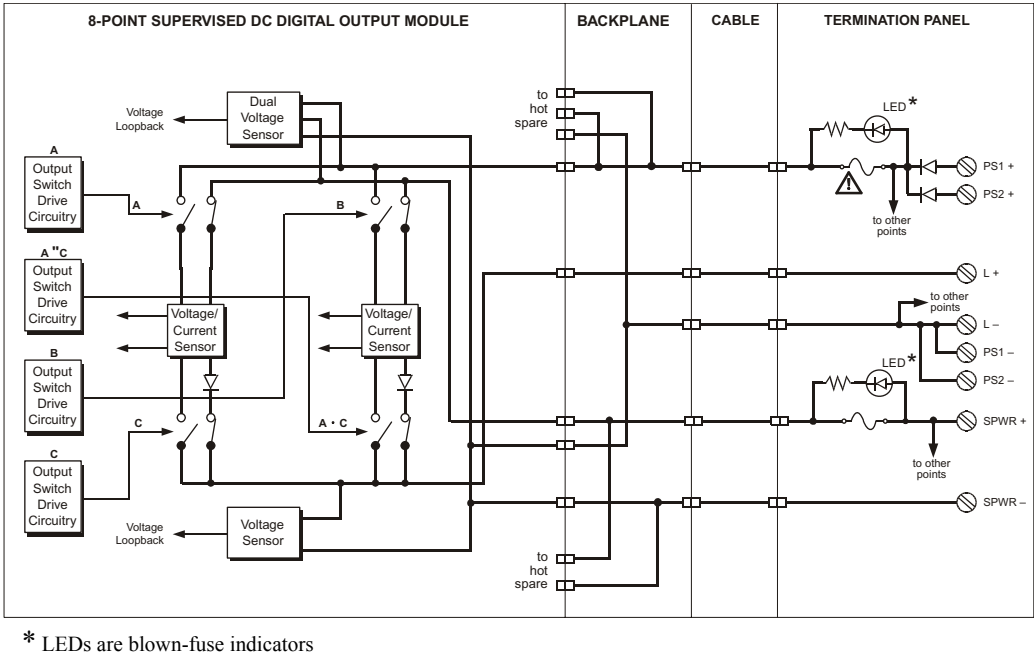
Figure 56 Simplified Schematic of a 3615E DO Module with a Commoned DO Panel
