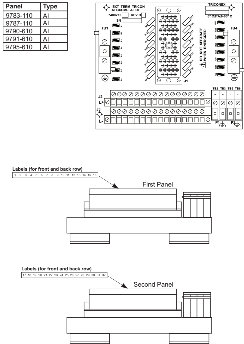
Figure 273 16-Point Commoned AI ATEX/RG 1.180 Label Placement
