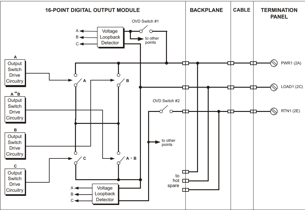
Figure 117 Simplified Schematic of a 3624 DO Module with a Basic DO Panel
