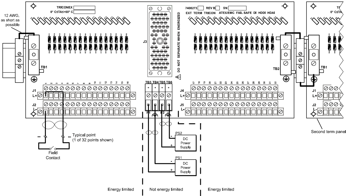
Figure 220 Field Wiring for 9570-610 with a 3504E DI Module
