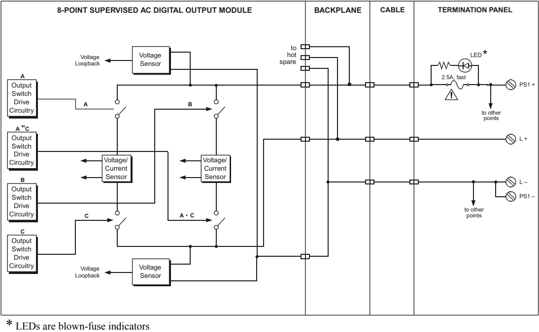
Figure 50 Simplified Schematic of a 3611E DO Module with a Commoned DO Panel
